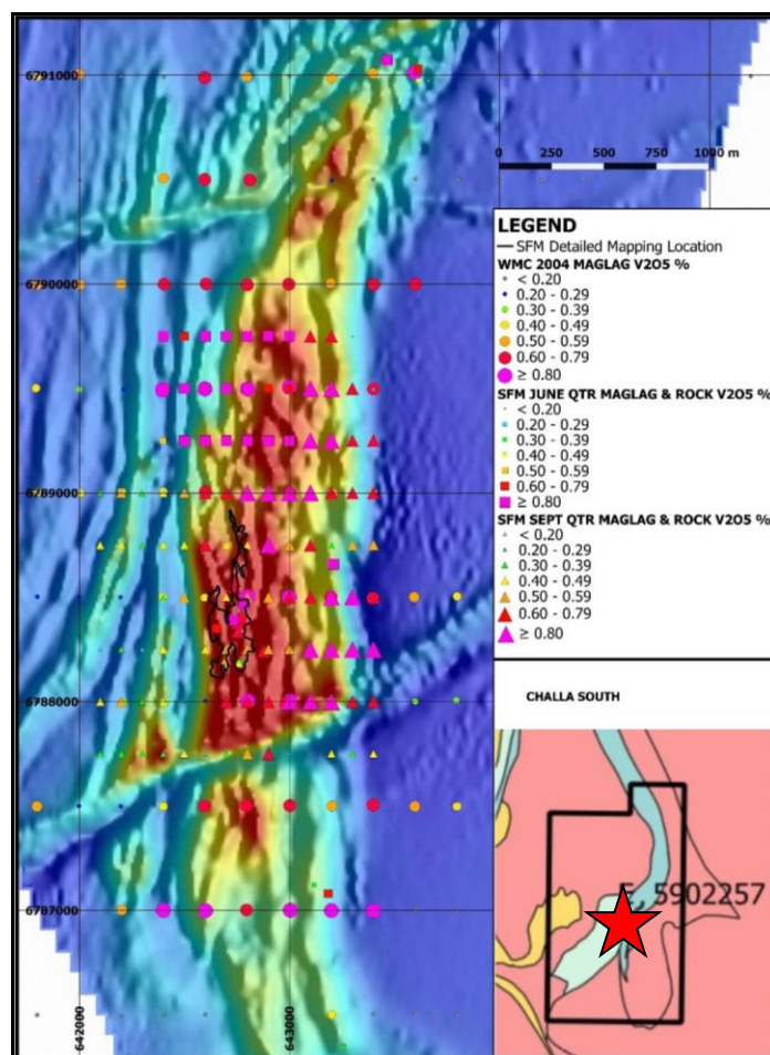
Figure 3 - V 2 O 5 MagLag and rock chip sampling assay results and location of detailed mapping location at Watson's Well Prospect
