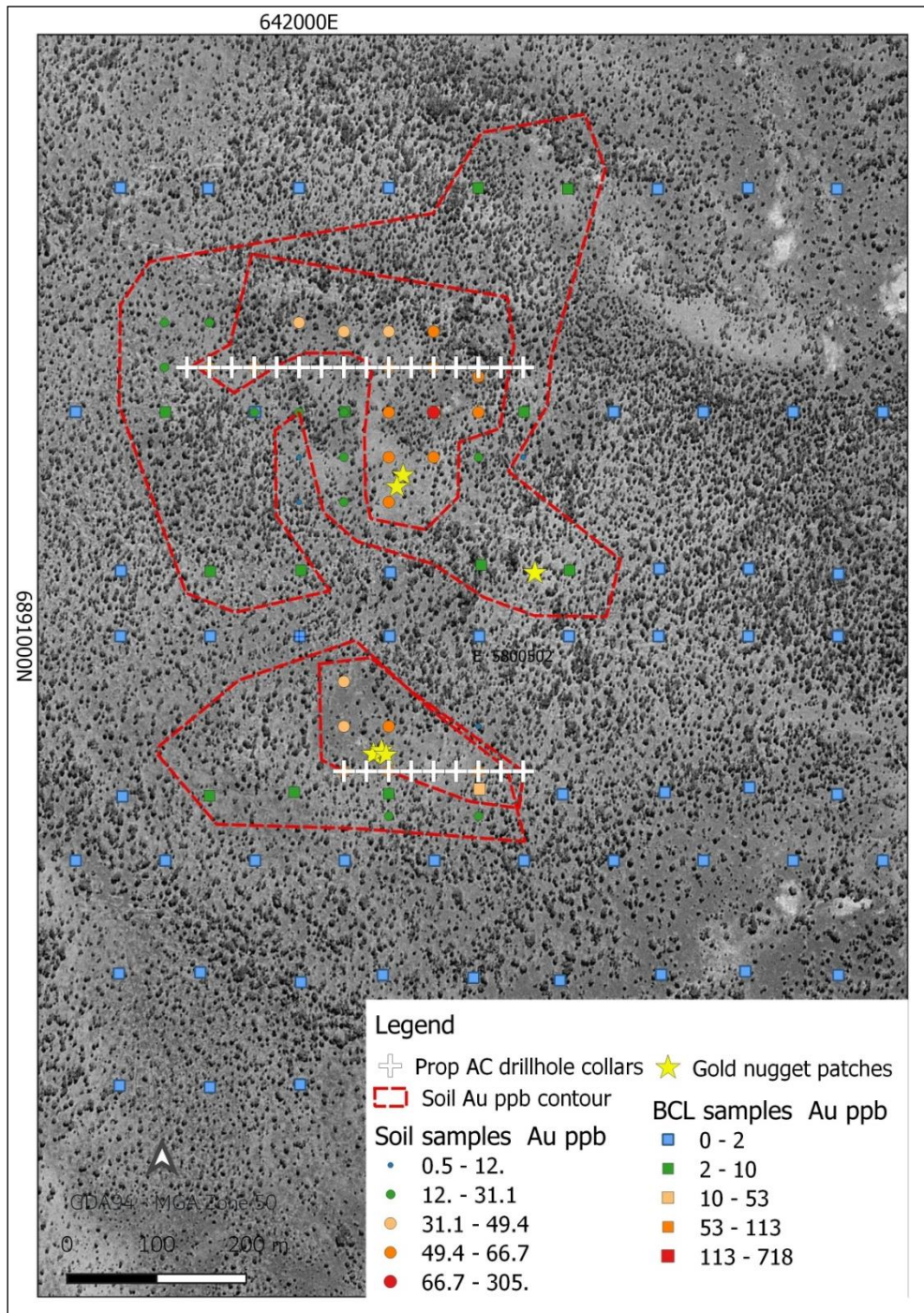
Figure 2 - Historic Brian's Patch soil geochemistry and proposed Aircore drill hole collars.
