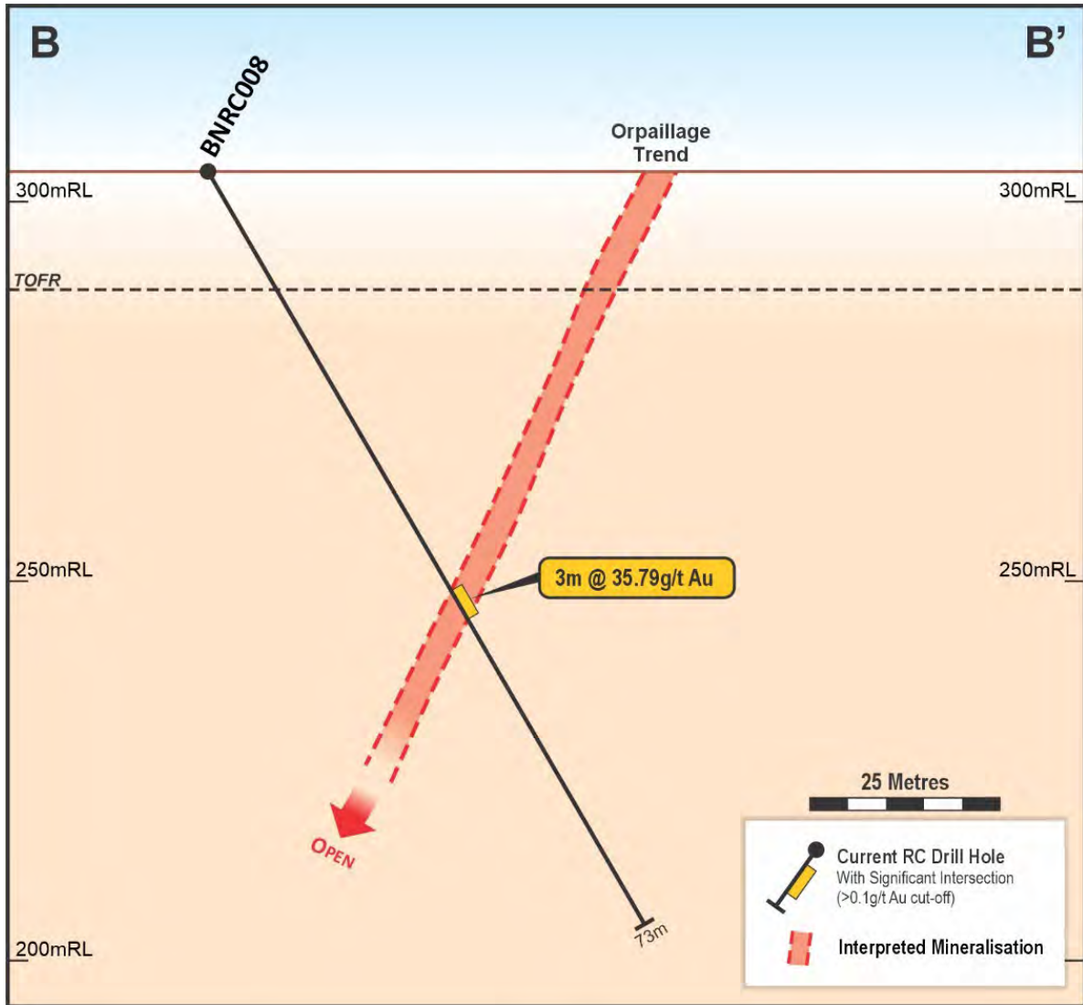
Figure 8 – Bouake North Cross section B-B' as referenced in figure 7.
